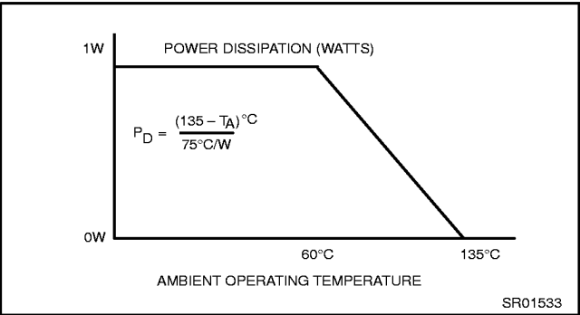
Figure 18. Power De-Rating Curve
