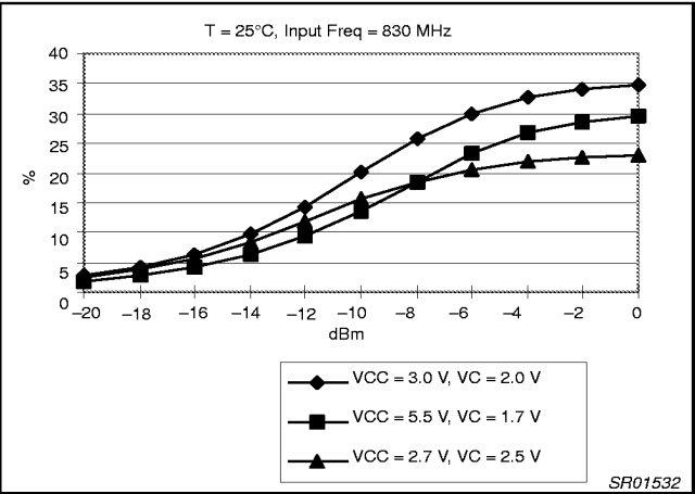
Figure 17. PAE VS Input Power
