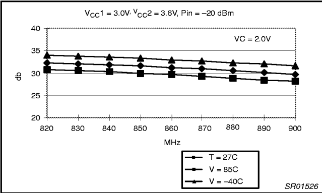
Figure 10. Signal Gain VS Input Frequency
