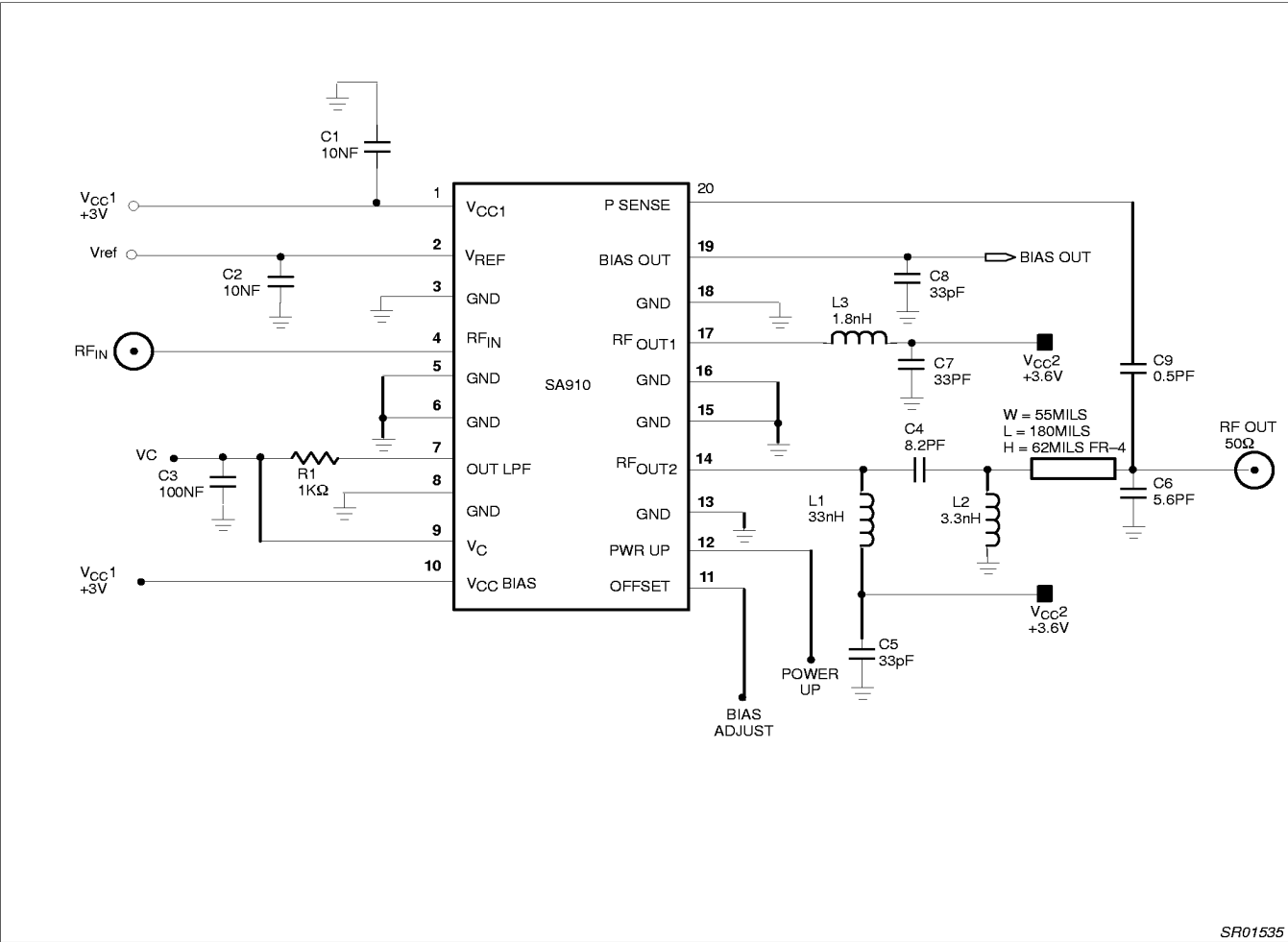
Figure 1. Application Diagram
