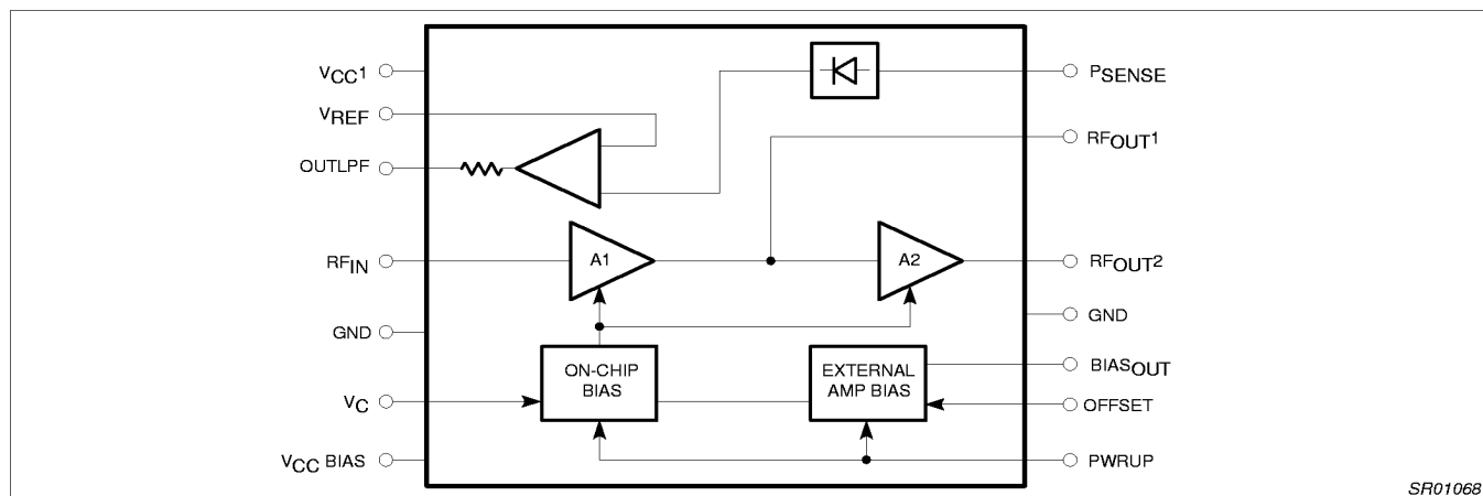
Figure 4. Block Diagram
