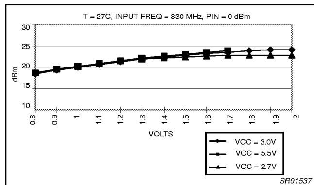
Figure 16. Output Power VS VREF (Closed Loop)
