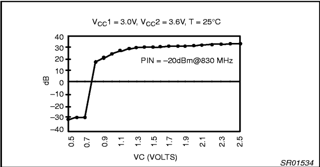
Figure 19. Small Signal Gain VS VC
