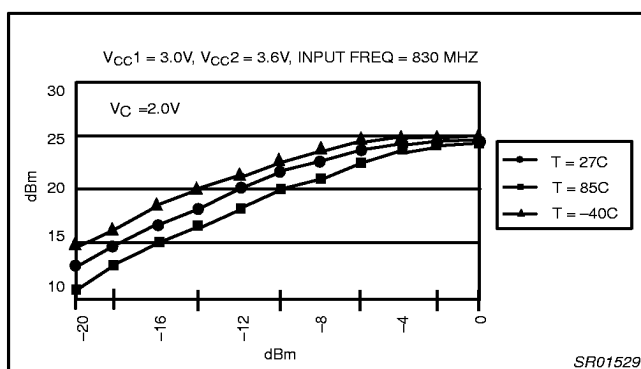
Figure 13. Output Power VS Input Power
