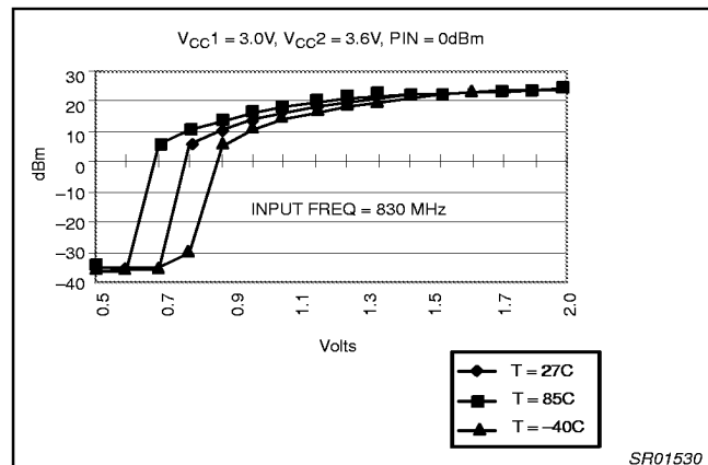
Figure 14. Output Power VS VC
