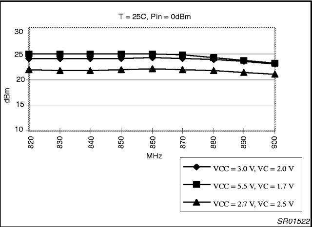
Figure 6. Output Power VS Input Frequency
