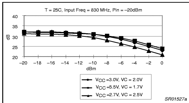
Figure 11. Signal Gain VS Input Power
