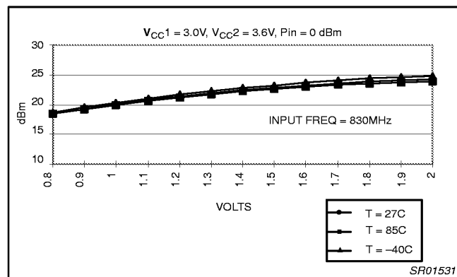
Figure 15. Output Power VS VREF (Closed Loop)
