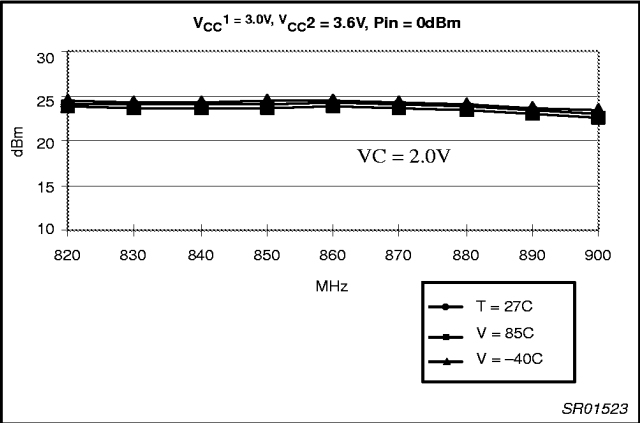
Figure 7. Output Power VS Input Frequency
