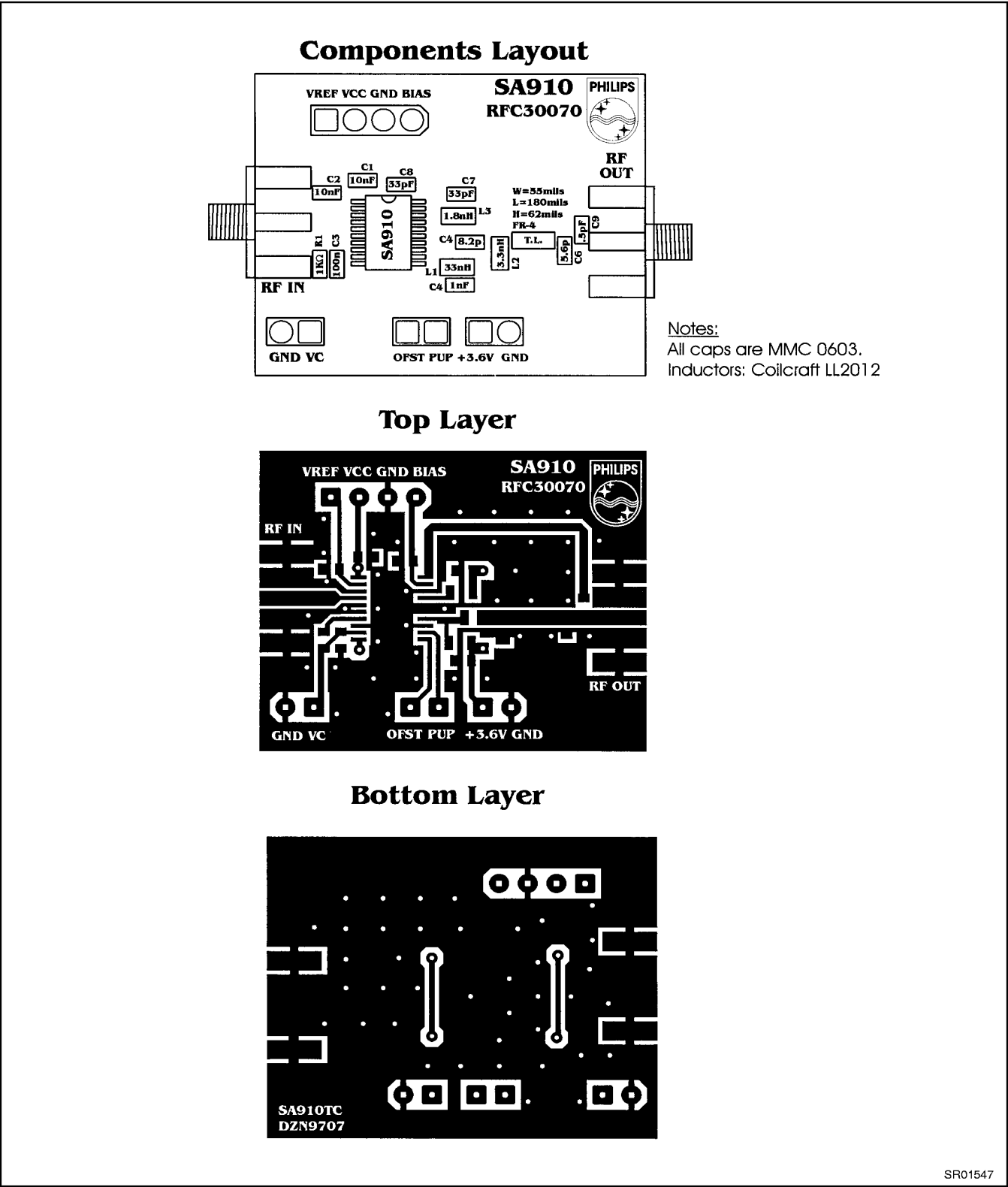
Figure 2. RF Predriver AMP
