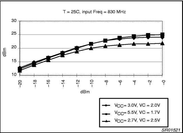
Figure 5. Output Power VS Input Power
