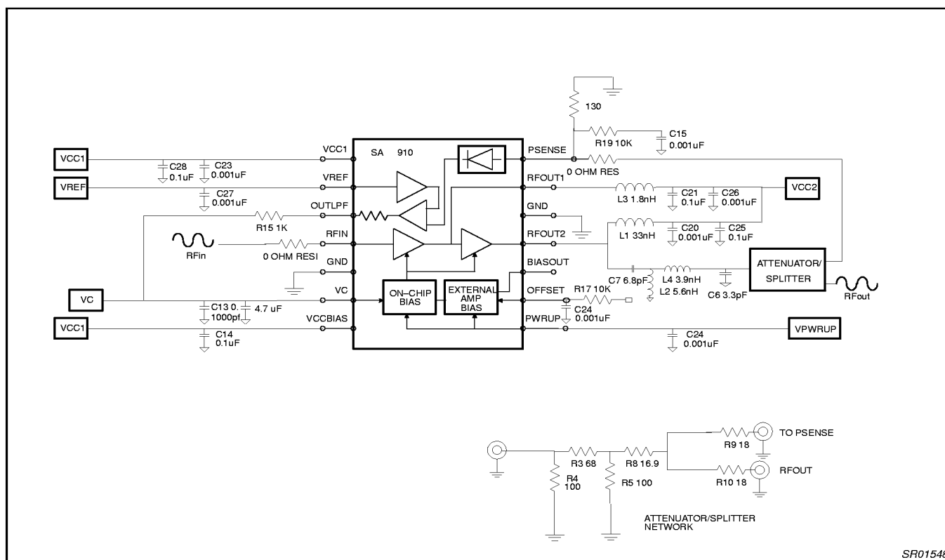
Figure 3. SA910 Test Circuit
