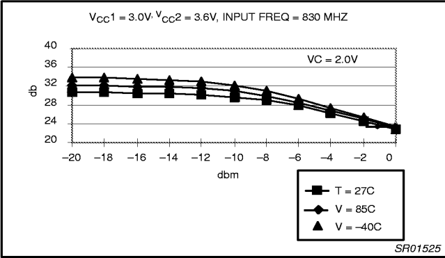
Figure 9. Signal Gain VS Input Power
