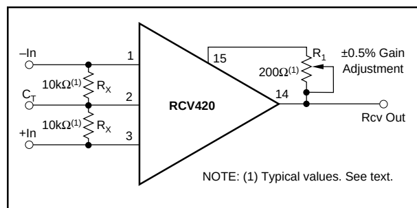
FIGURE 2. Optional Gain Adjustment.
