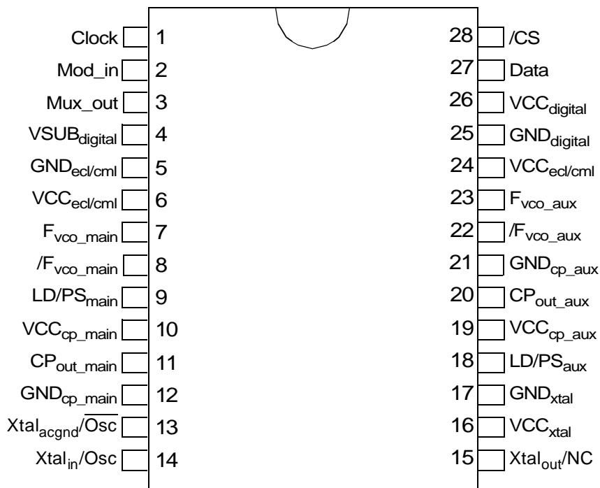
Figure 3: PS1200 Pinout.
