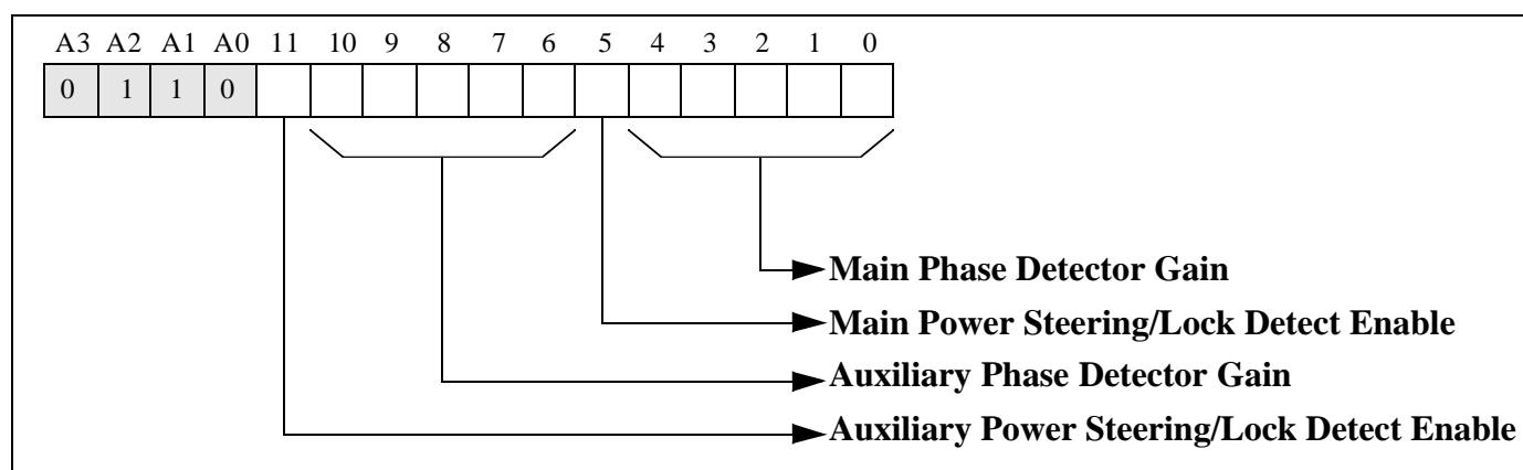
Figure 10: Hex6 Phase Detectors Register (Write only)
