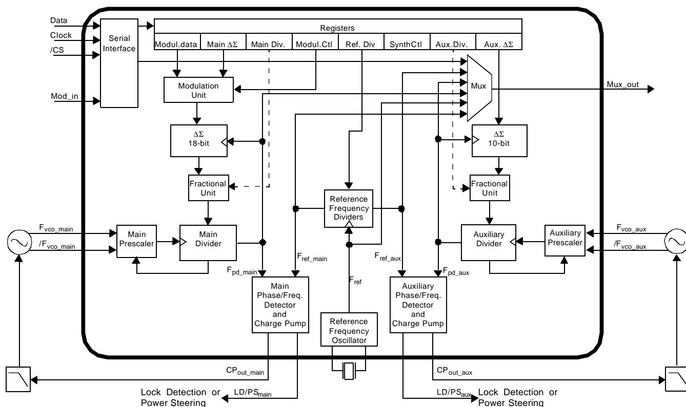
Figure 1: PS1200 Block Diagram
