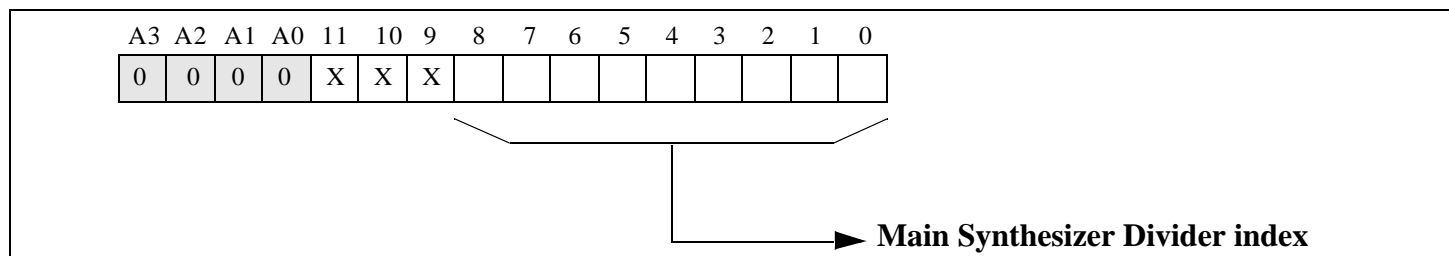
Figure 4: Hex0 Main Divider Register (Write only)
