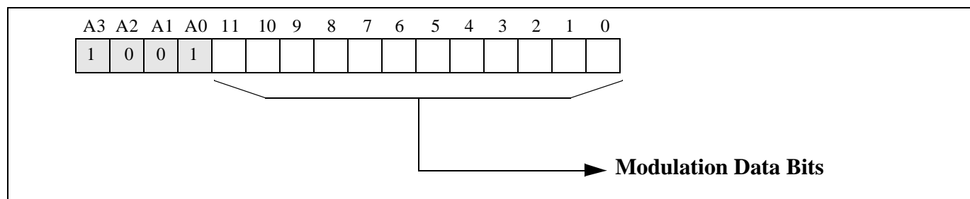
Figure 13: Hex9 Modulation Data Register (Write only)
