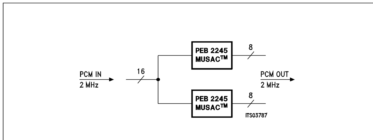
Figure 6 Memory Time Switch 16/16 for a Non-Blocking 512-Channel Switch with Conferencing Capability
