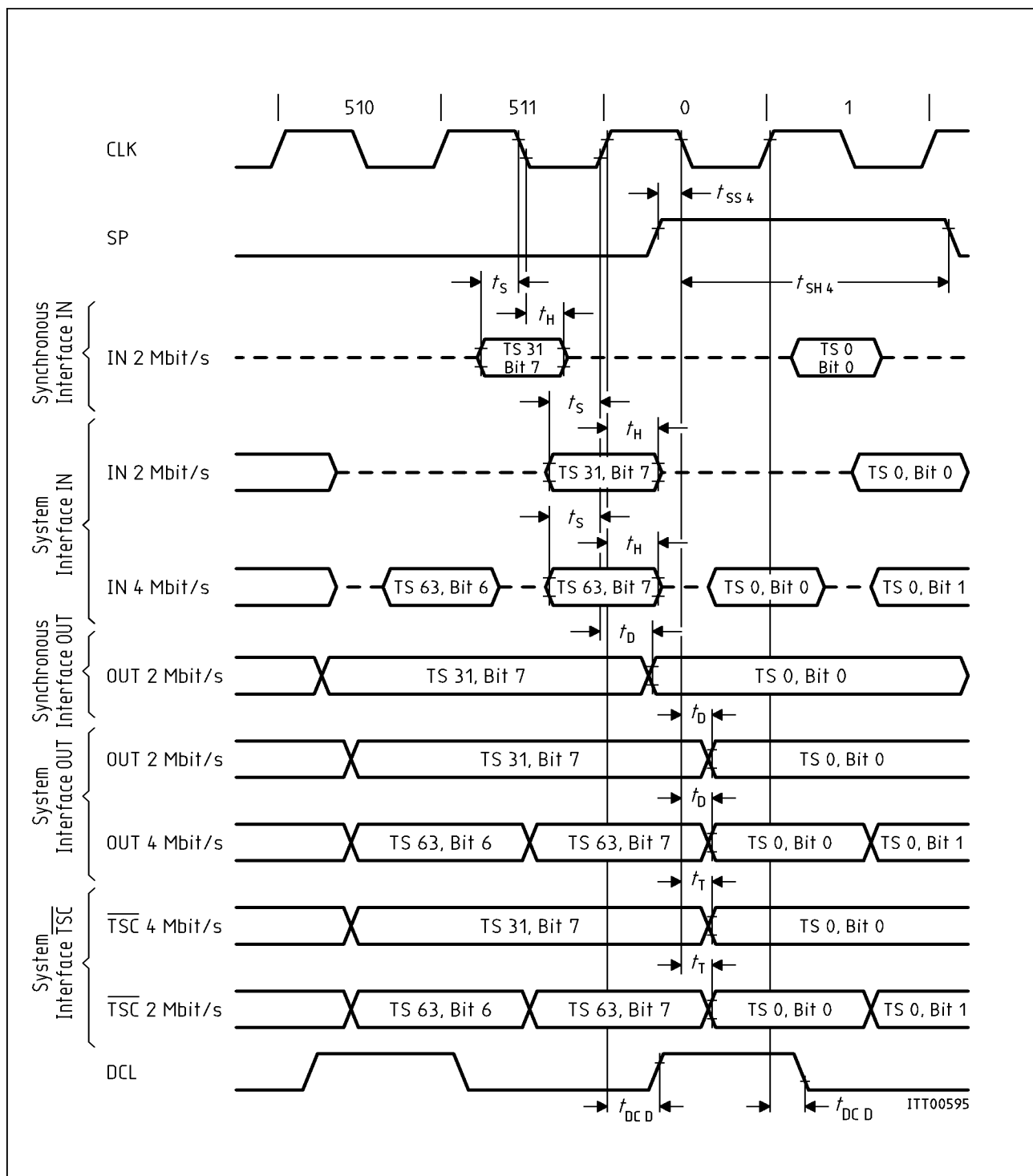
Figure 28 PCM-Line Timing in Primary Access Configuration with a 4-MHz Device Clock and a CSR Entry (00010001)
