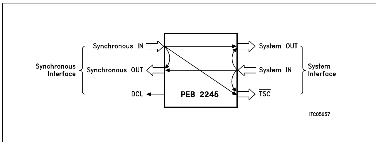
Figure 14 Connection Choices in the Primary Access Configuration
