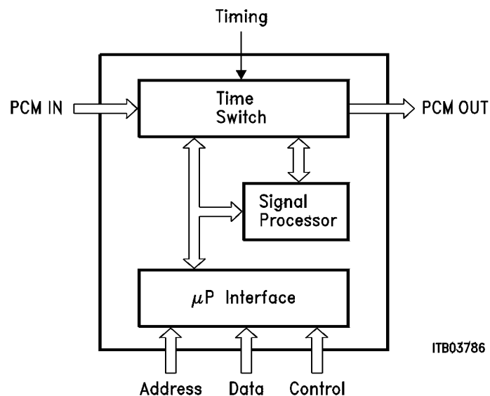
Figure 5 Block Diagram of the PEB 2245
