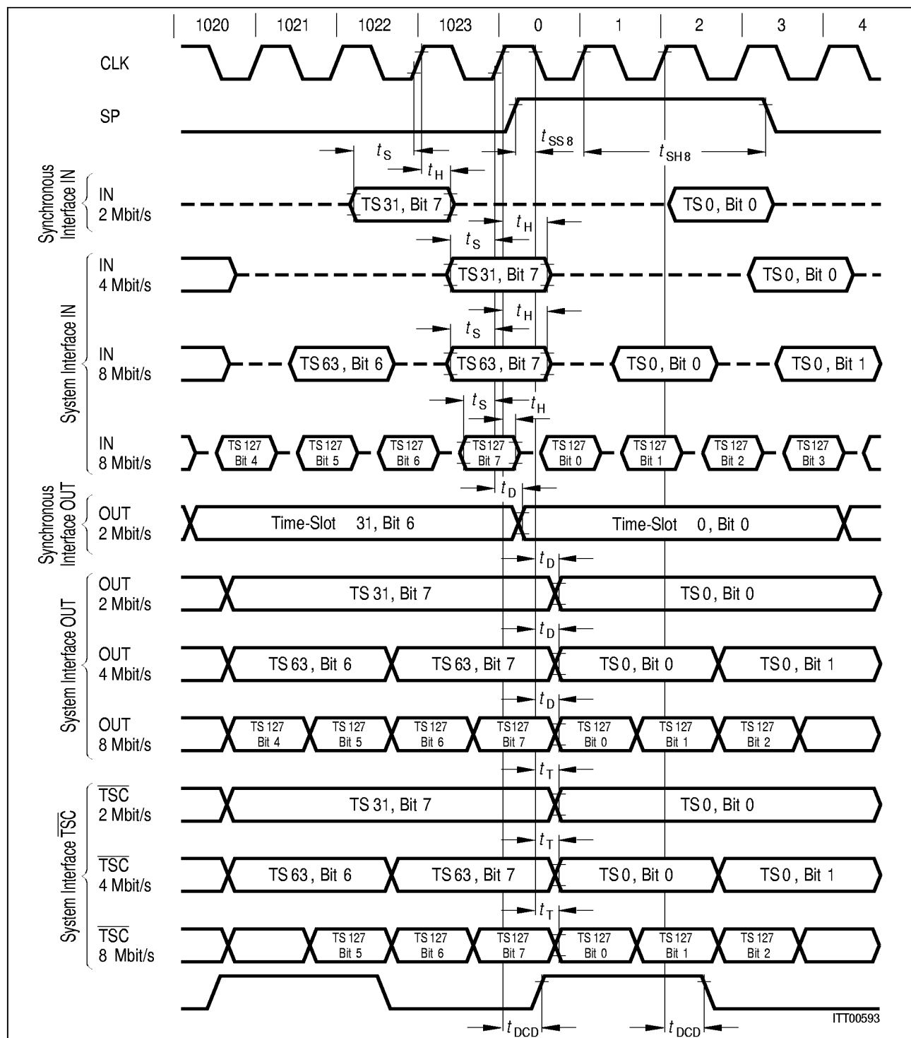
Figure 26 PCM-Line Timing in Primary Access Configuration with a 8-MHz Device Clock and a CSR Entry (00010001)
