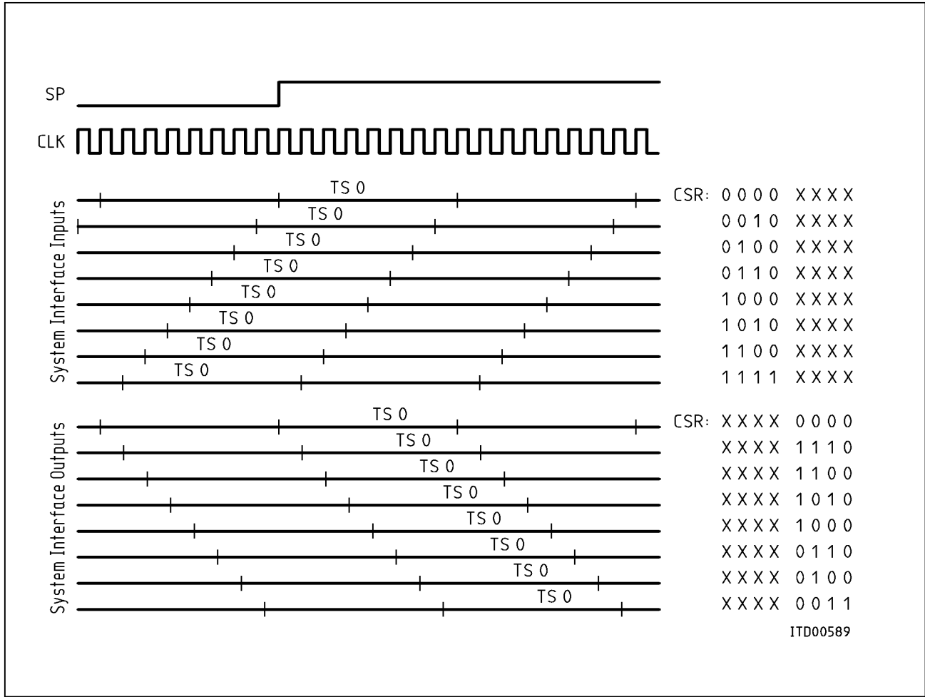
Figure 19 Clock Shifting
