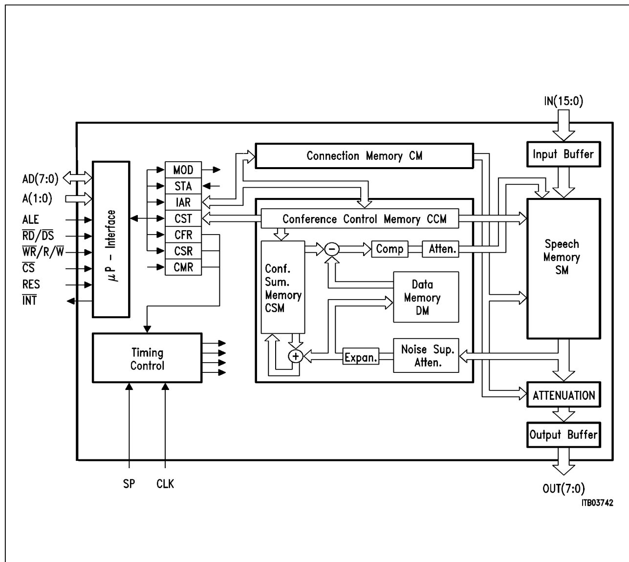
Figure 10 Detailed Block Diagram of the PEB 2245
