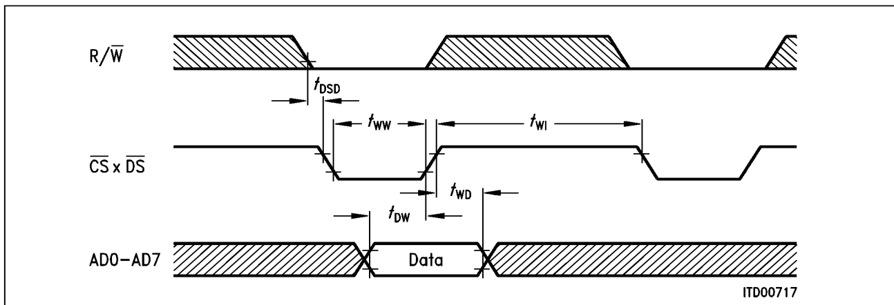
Figure 23 Multiplexed Address Timing
