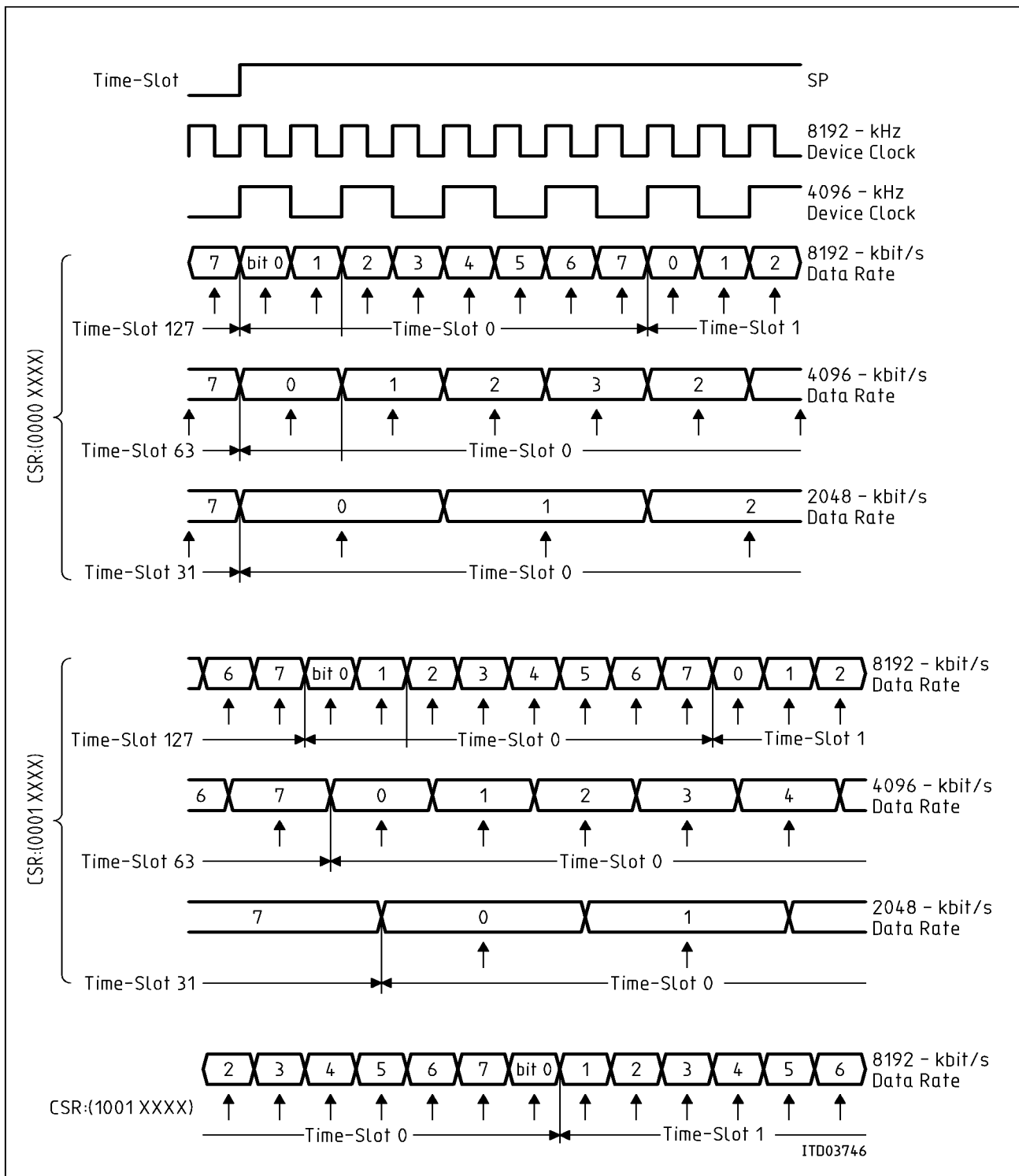
Figure 11 Latching Instant for Input Data
