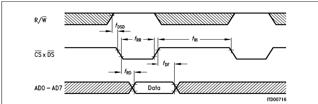
Figure 22 \mu P Write Cycle
