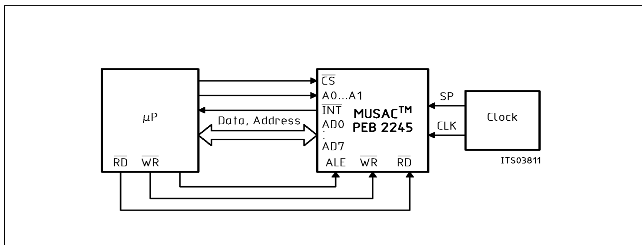
Figure 15 The MUSAC™ Controlled by a Intel Microprocessor
