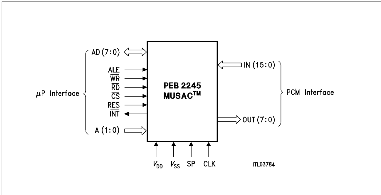
Figure 3 Functional Symbol for the Standard Configuration
