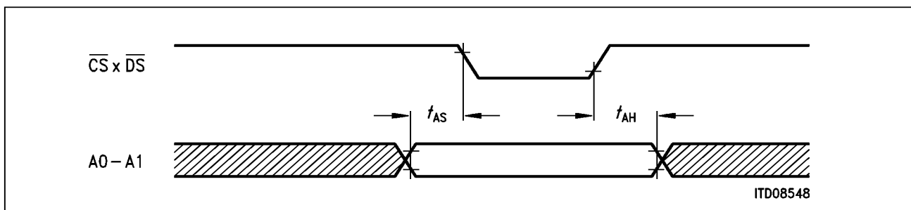
Figure 24 Non-multiplexed Address Timing
