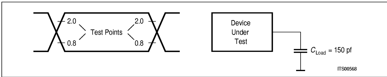
Figure 20 I/O Waveform for AC Tests
