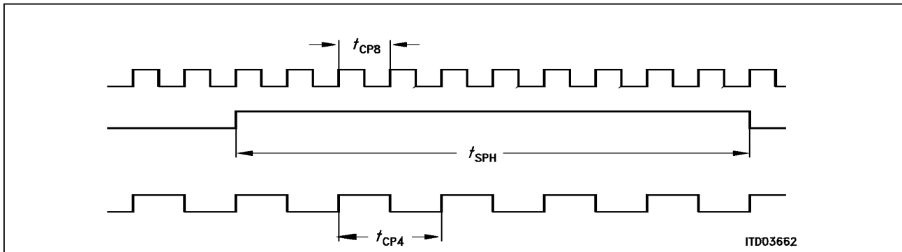
Figure 13 SYP Duration for N = 2
