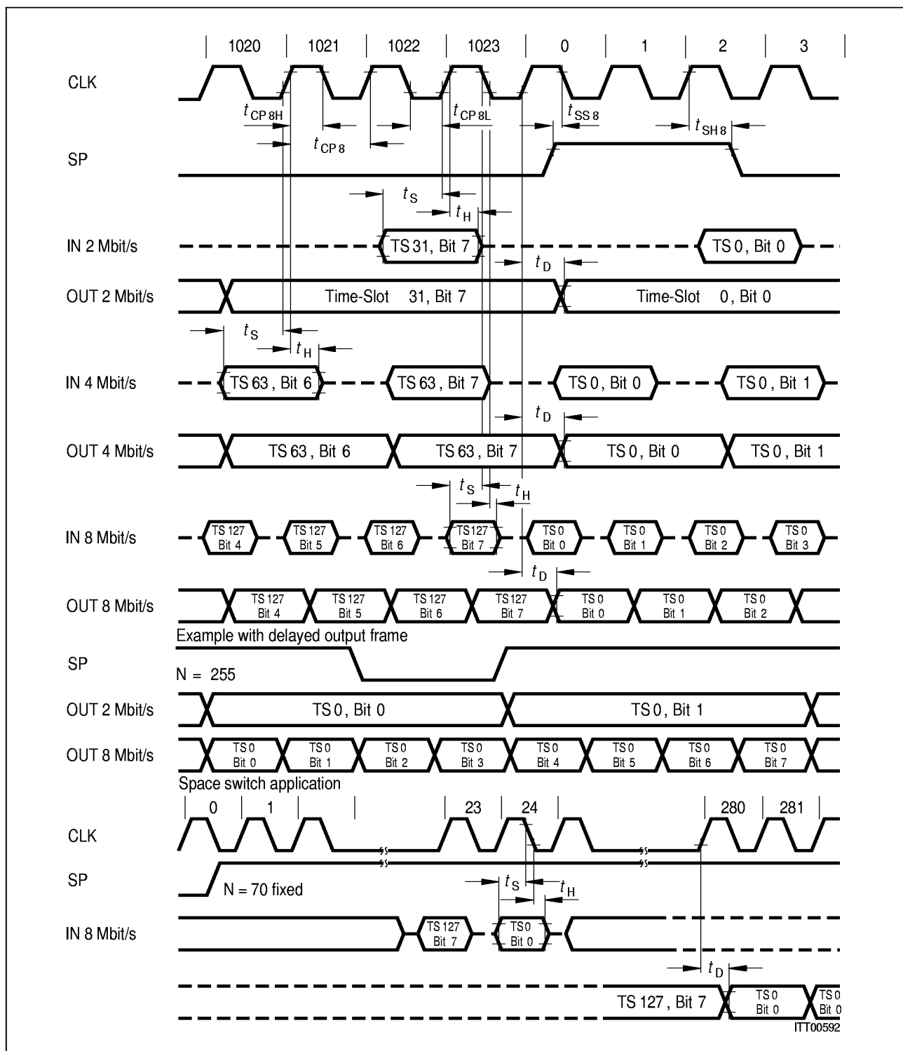
Figure 25 PCM-Line Timing in Standard Configuration with a 8-MHz Device Clock
