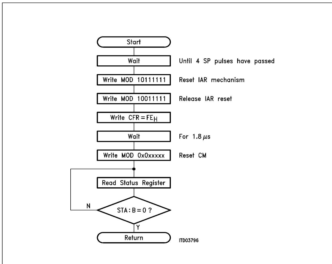
Figure 18 Initializing the PEB 2245 for a 4096-kHz Device Clock
