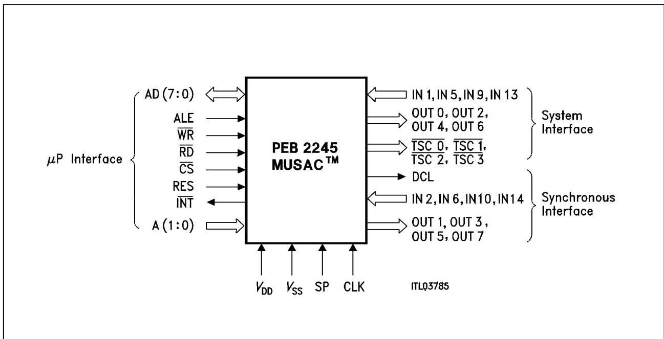
Figure 4 Functional Symbol for the Primary Access Configuration
