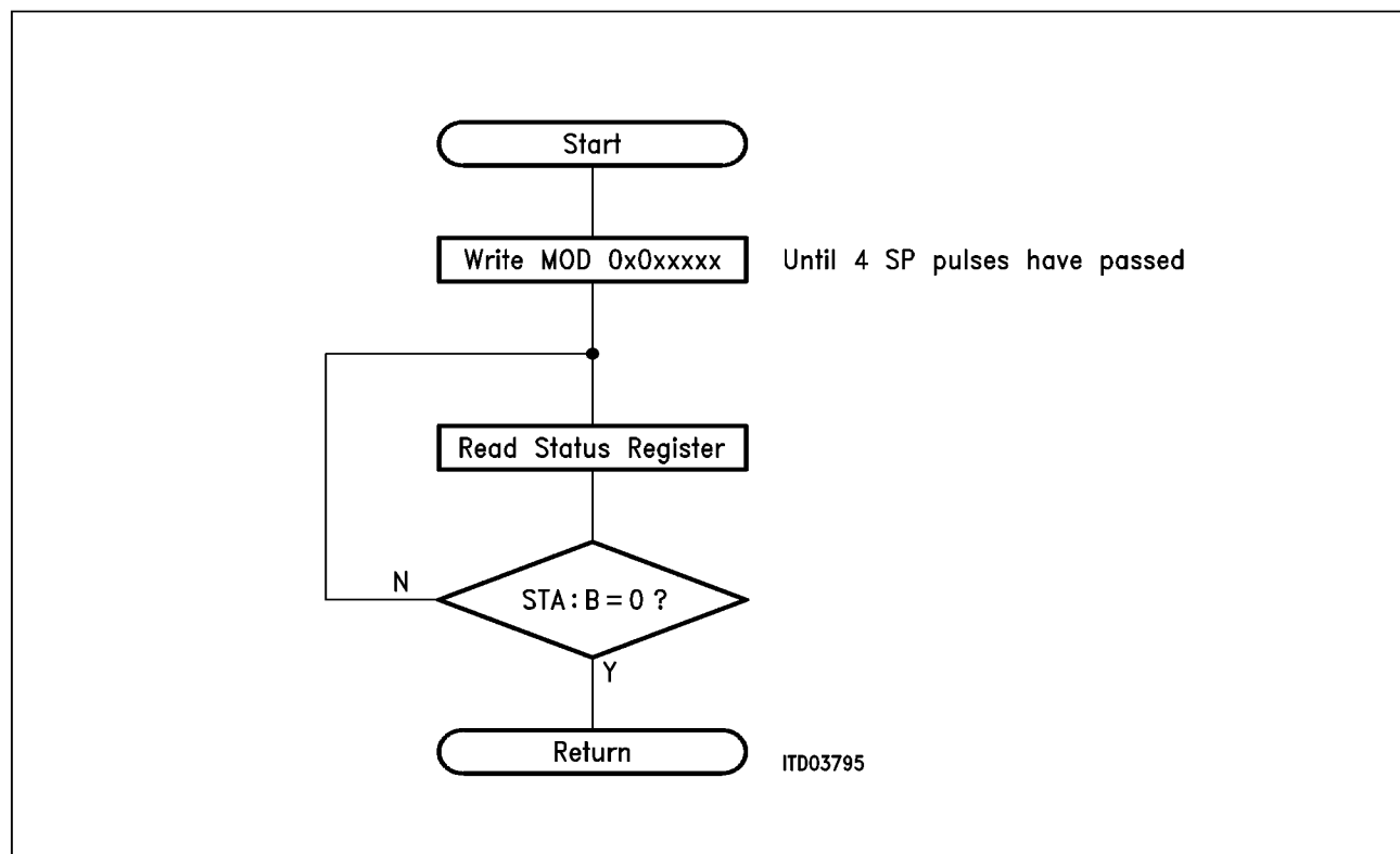
Figure 17 Initializing the PEB 2245 for a 8192-kHz Device Clock
