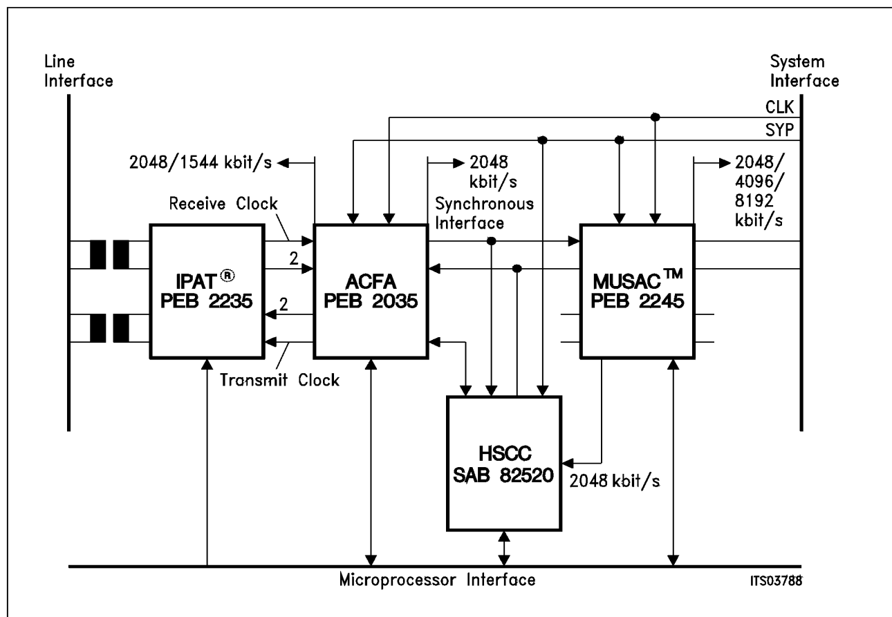
Figure 7 Architecture of a Primary Access Board
