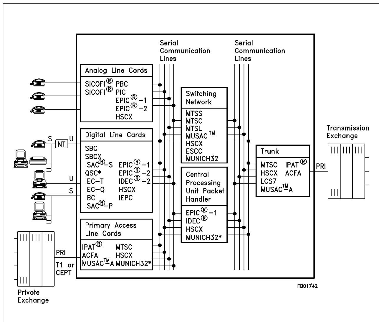
Figure 1 General Exchange Architecture
