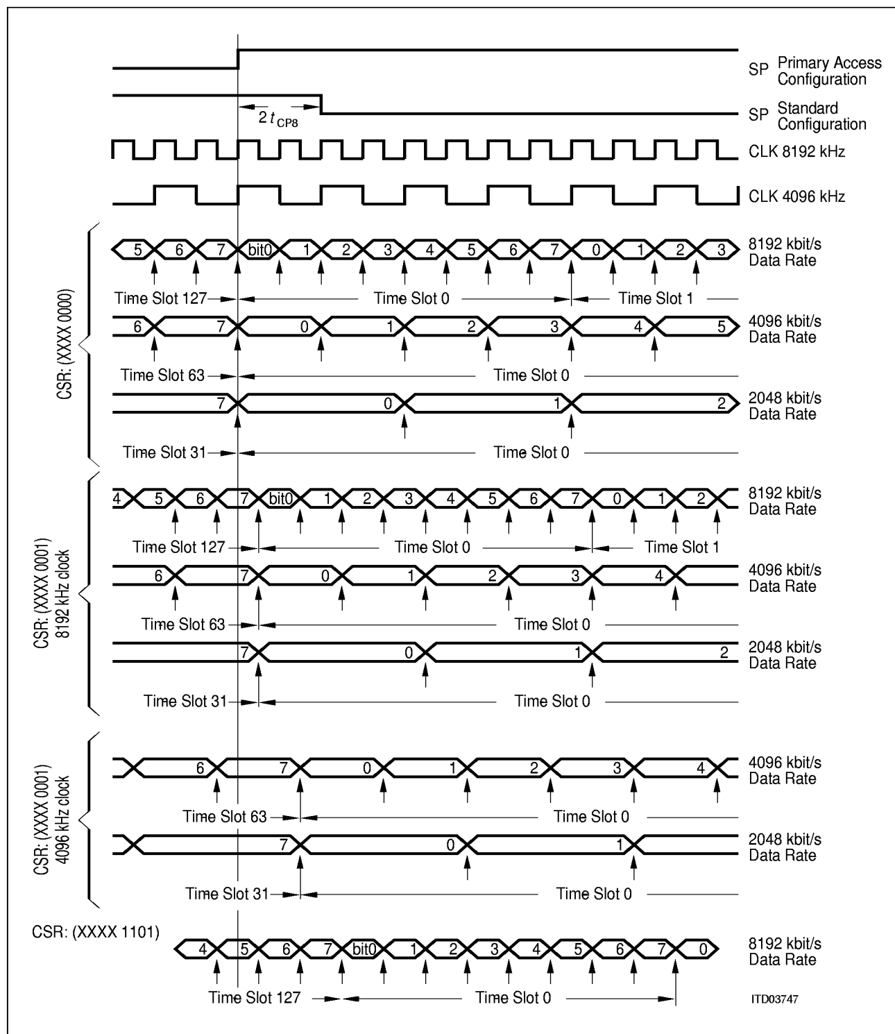
Figure 12 Clocking Off Instant of Output Data
