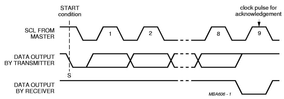
Fig.11 Acknowledgement on the I 2 C-bus.
