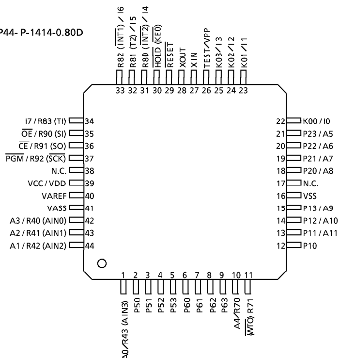
QFP44-P-1414-0.80D
