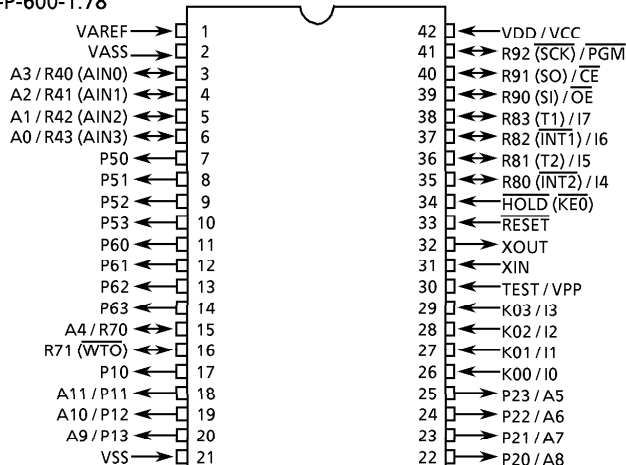
SDIP42-P-600-1.78
