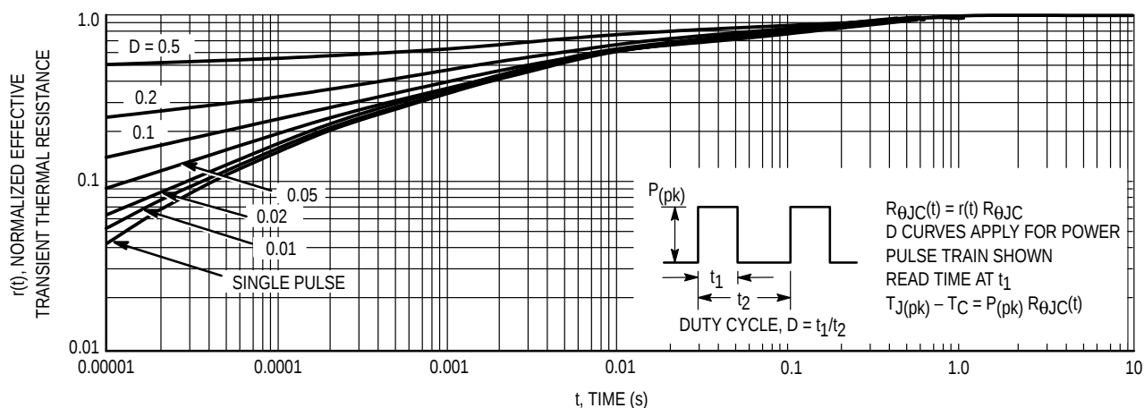
Figure 13. Thermal Response
