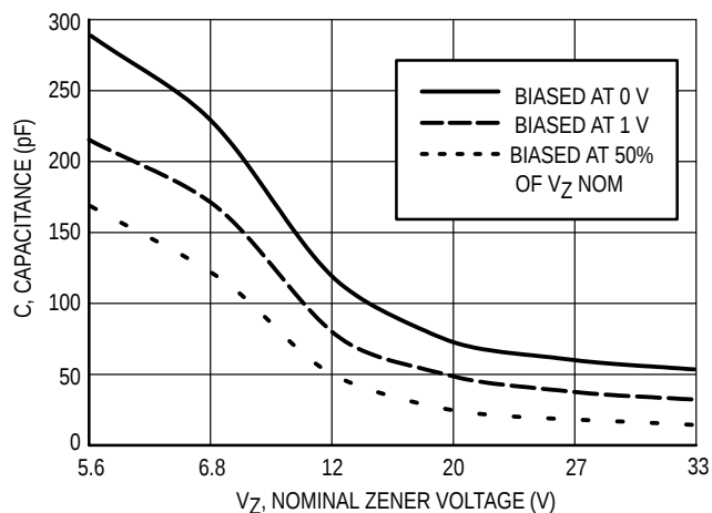
Figure 1. Typical Capacitance
