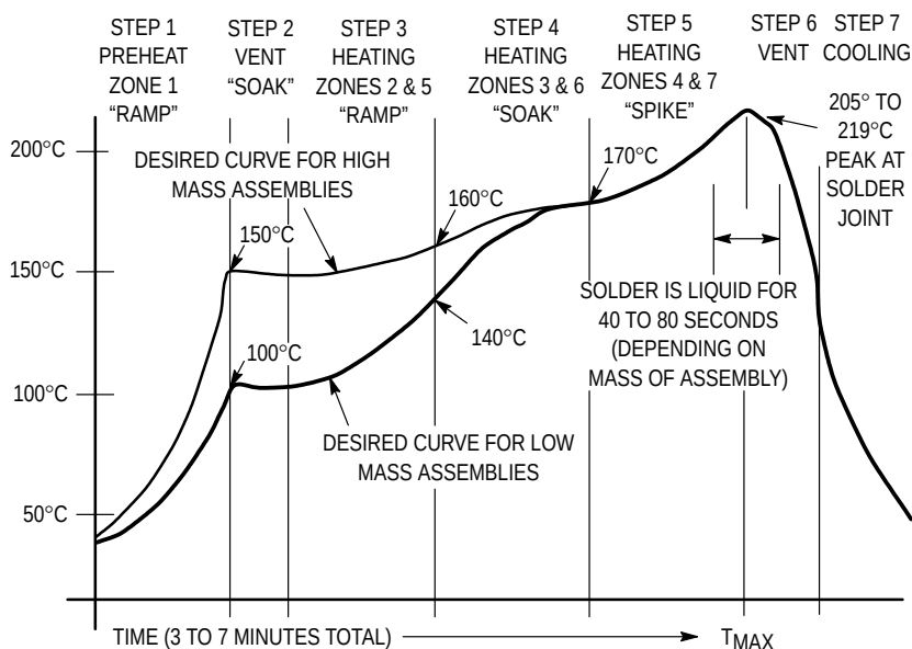
Figure 16. Typical Solder Heating Profile
