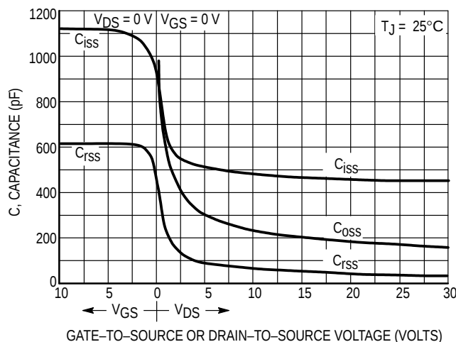
Figure 8. Capacitance Variation
