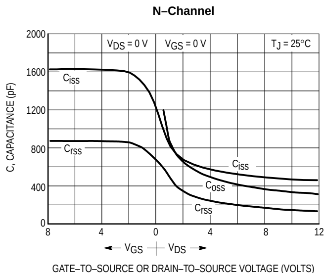
Figure 7. Capacitance Variation
