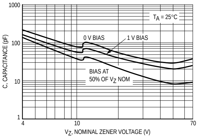
Figure 3. Typical Capacitance
