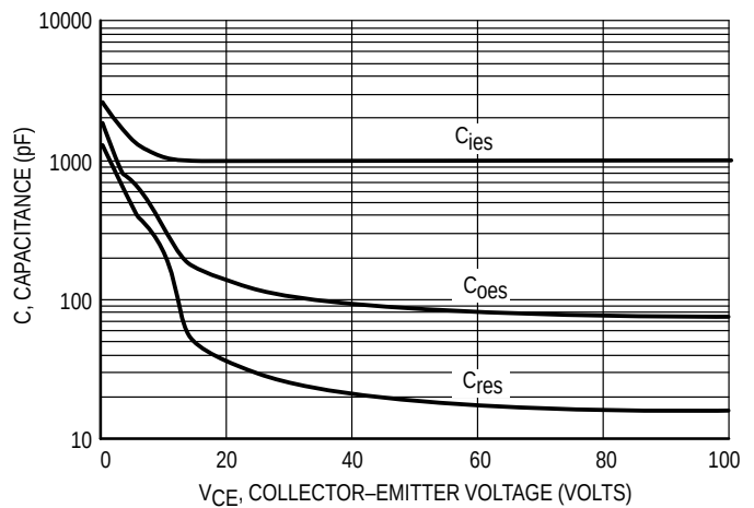
Figure 16. Capacitance Variation
