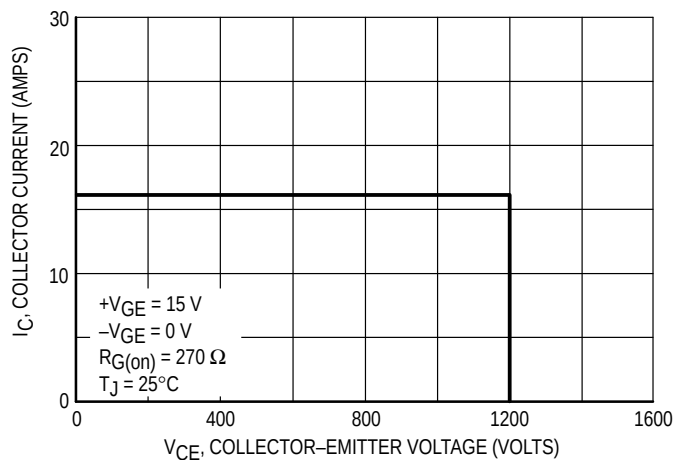
Figure 17. Reversed Biased Safe Operating Area (RBSOA)
