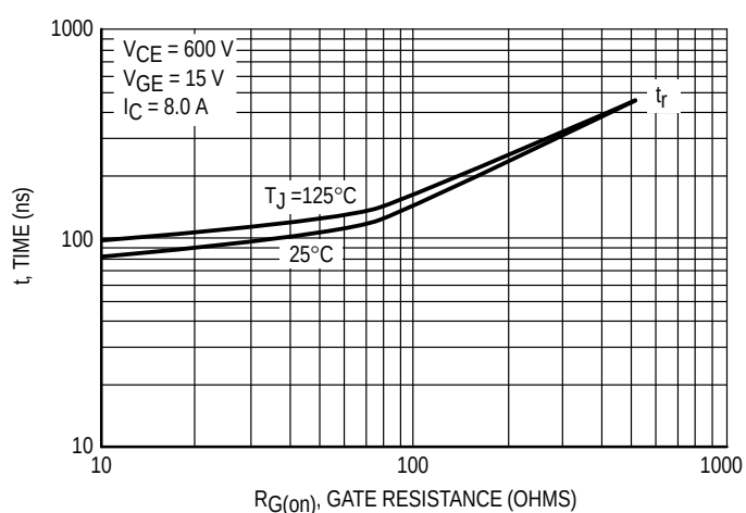
Figure 12. Inductive Switching Times versus Gate Resistance
