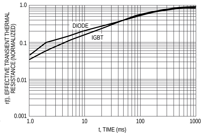
Figure 18. Thermal Response
