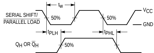
Figure 2. Parallel-Load Mode
