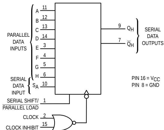
LOGIC DIAGRAM
