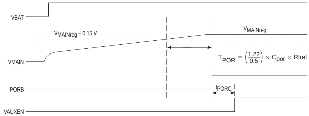
Figure 2. Startup Timing
