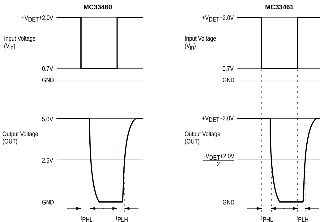
Figure 1. T_{pd} Measurement Conditions
