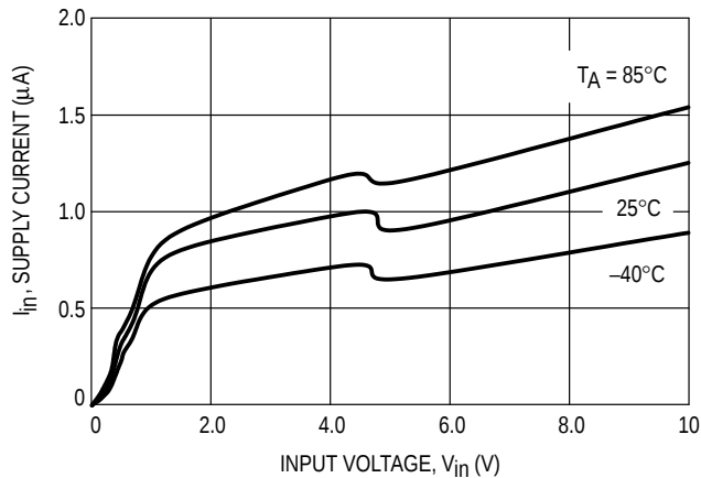
Figure 2. Supply Current vs. Input Voltage
