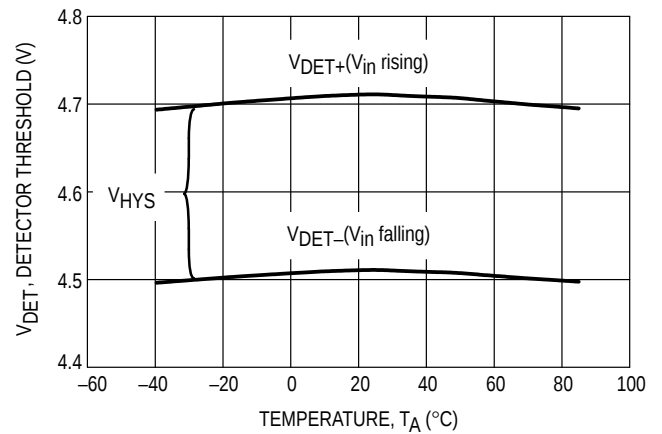
Figure 3. Detector Threshold Hysteresis vs. Temperature
