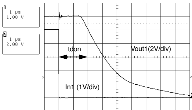
Figure 18 - Turn on Delay
