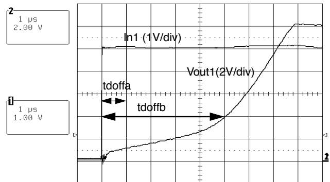
Figure 19 - Turn off Delay
