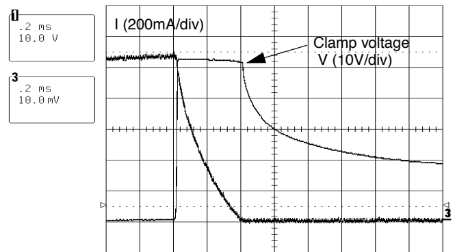
Figure 17 - Inductive Switching
