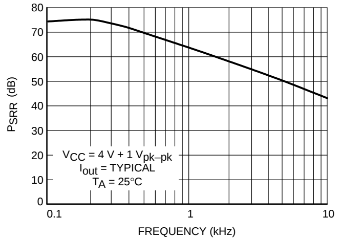
Figure 8. PSRR versus Frequency (All Regulators)
