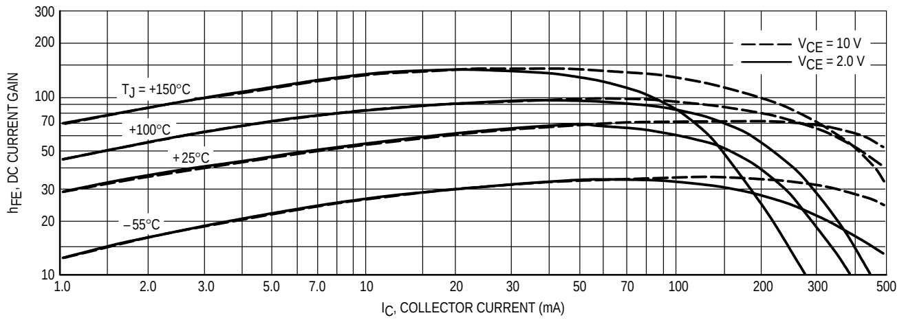
Figure 4. Current Gain
