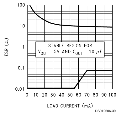
FIGURE 2. 5V/10 \mu F ESR Curves
