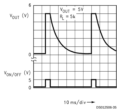
Turn-Off Waveform
