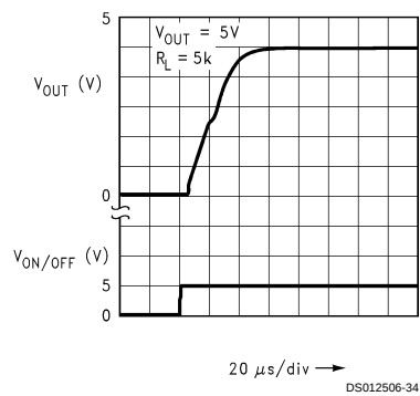
Turn-On Waveform
