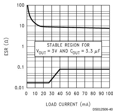
FIGURE 3. 3V/3.3 \mu F ESR Curves
