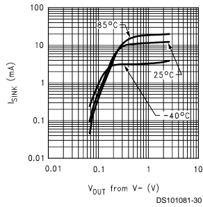
Sinking Current vs. V_{OUT} V^+ = 2.7V
