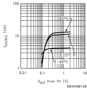
Source Current vs. Out V^+ = 2.7V
