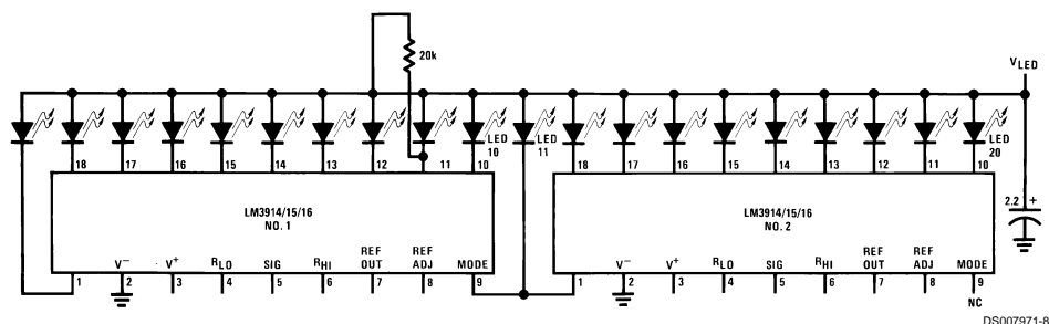
FIGURE 1. Cascading LM3914/15/16 Series in Dot Mode
