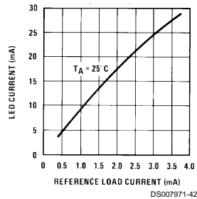
LED Current vs Referenced Loading
