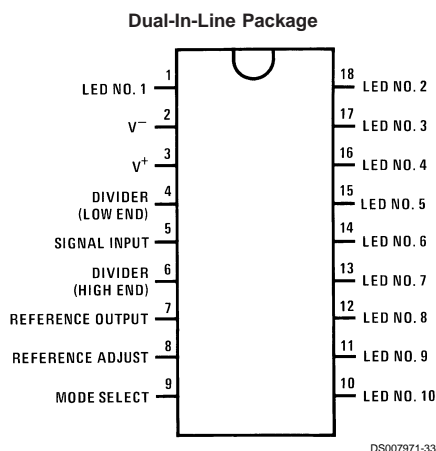
Top View Order Number LM3916N See NS Package Number N18A
