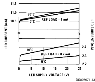
LED Driver Current Regulation
