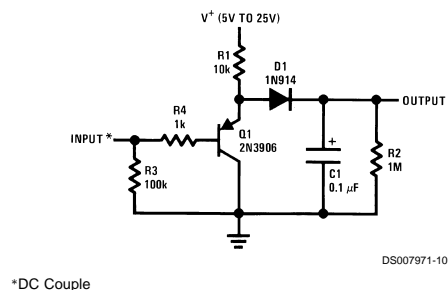
FIGURE 3. Half-Wave Peak Detector
