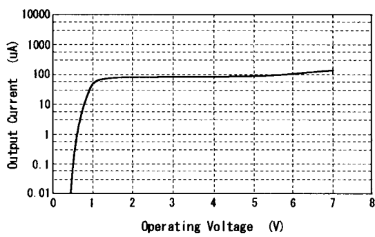
Output Current vs. Operating Voltage VIN=0.1V
