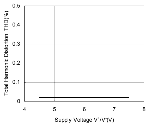
Total Harmonic Distortion vs. Supply Voltage ( V_{in}=1\text{kHz}/1.25\text{V}_{pp} , T_a=25^\circ\text{C} )
