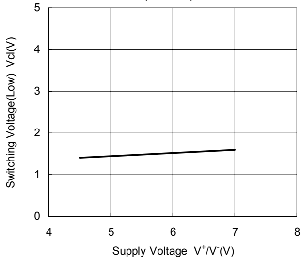
Switching Voltage(Low) vs. Supply Voltage ( T_a=25^\circ\text{C} )
