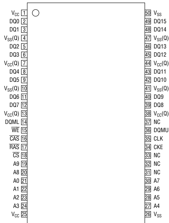
50-Pin Plastic TSOP (II) (K Type)
