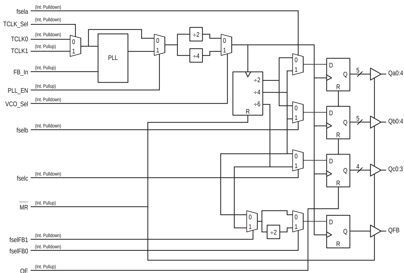
Figure 2. Logic Diagram
