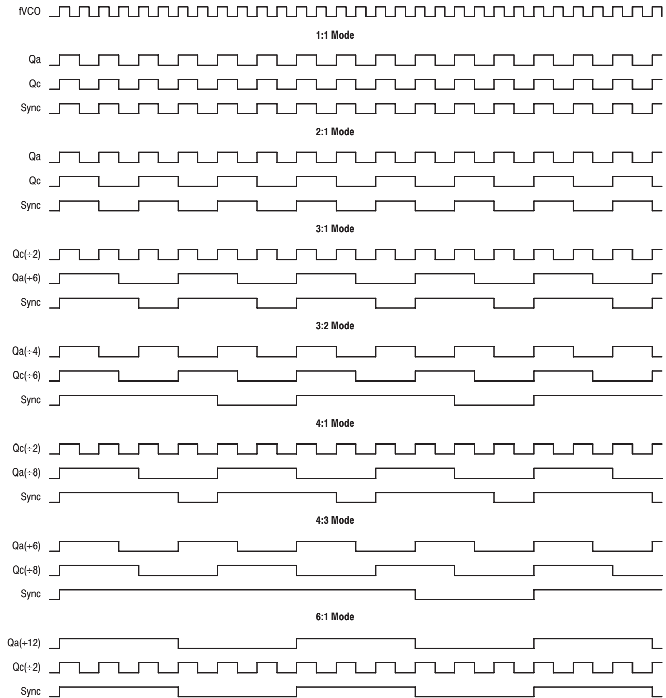
Figure 3. Timing Diagrams
