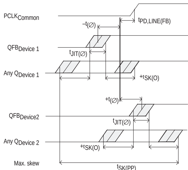
Figure 4. MPC9653 max. device-to-device skew
