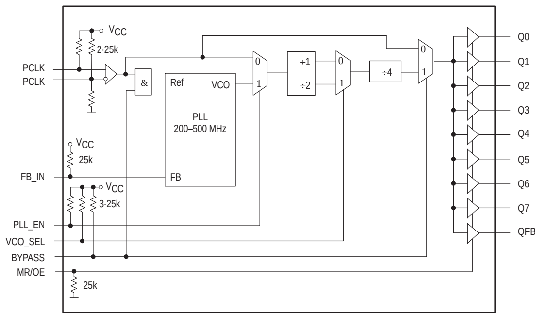
Figure 1. MPC9653 Logic Diagram
