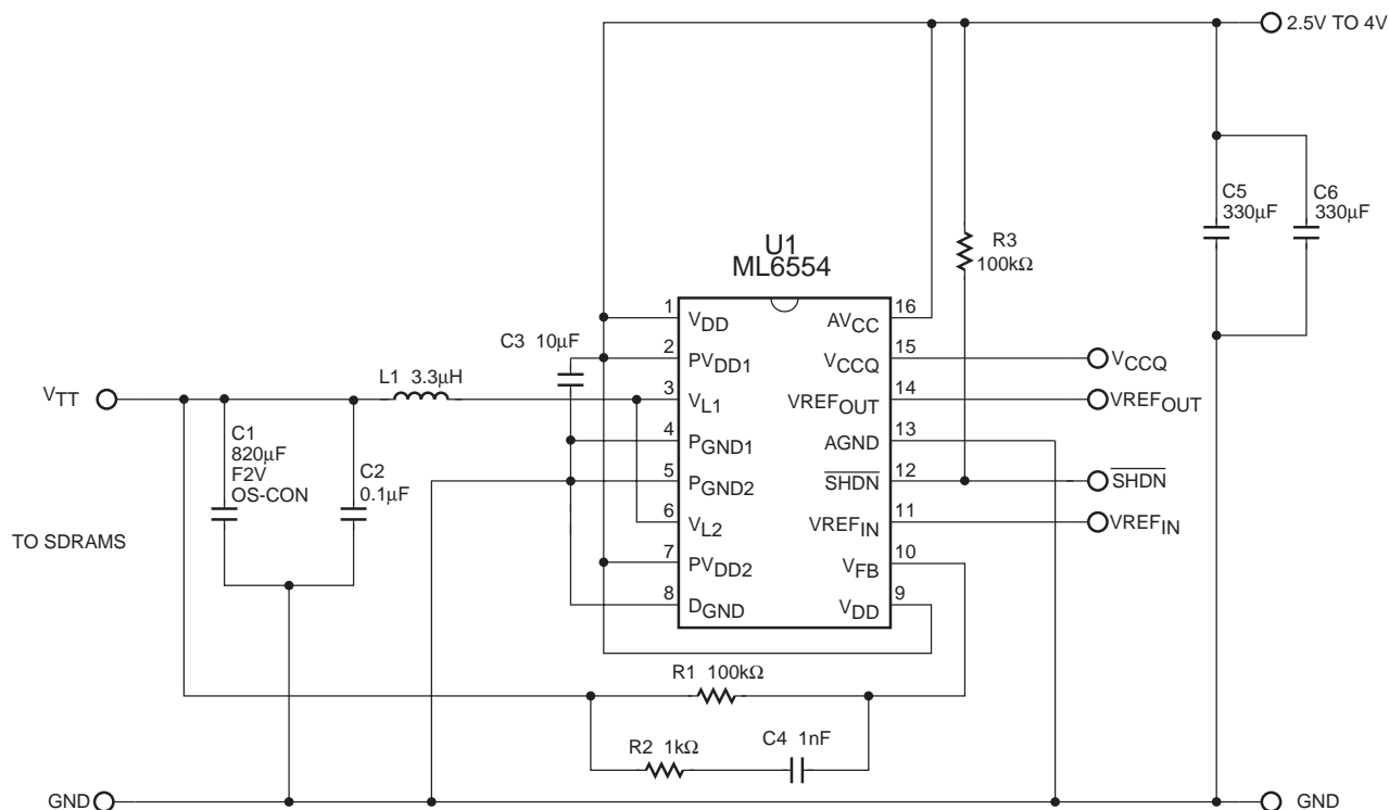
Figure 3. Alternate Application Circuit
