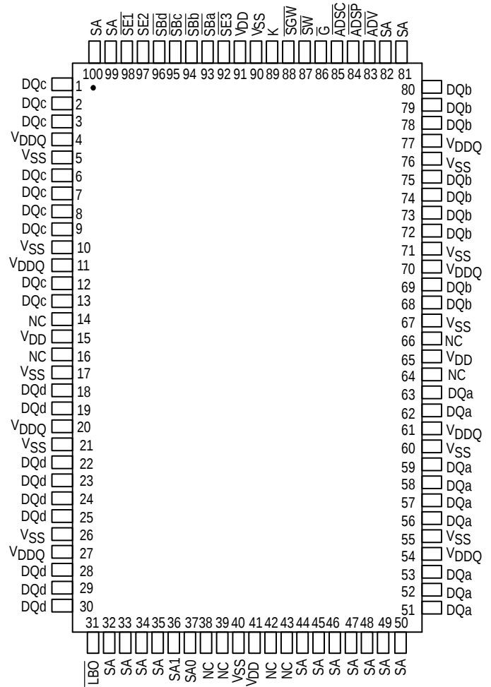
TOP VIEW 100 PIN TQFP
