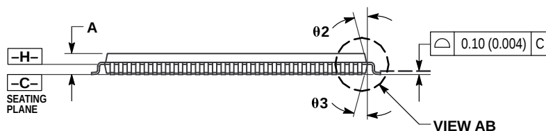
NOTES: 1. DIMENSIONING AND TOLERANCING PER ANSI Y14.5M, 1982. 2. CONTROLLING DIMENSION: MILLIMETER. 3. DATUM PLANE --H-- IS LOCATED AT BOTTOM OF LEAD AND IS COINCIDENT WITH THE LEAD WHERE THE LEAD EXITS THE PLASTIC BODY AT THE BOTTOM OF THE PARTING LINE. 4. DATUMS --A--, --B-- AND --D-- TO BE DETERMINED AT DATUM PLANE --H--. 5. DIMENSIONS D AND E TO BE DETERMINED AT SEATING PLANE --C--. 6. DIMENSIONS D1 AND E1 DO NOT INCLUDE MOLD PROTRUSION. ALLOWABLE PROTRUSION IS 0.25 (0.010) PER SIDE. DIMENSIONS D1 AND B1 DO INCLUDE MOLD MISMATCH AND ARE DETERMINED AT DATUM PLANE --H--. 7. DIMENSION B DOES NOT INCLUDE DAMBAR PROTRUSION. DAMBAR PROTRUSION SHALL NOT CAUSE THE b DIMENSION TO EXCEED 0.45 (0.018).
