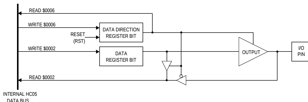
Figure 6-3. Port C I/O Circuitry
