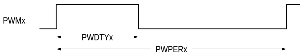
Figure 8-5. PWM duty cycle
