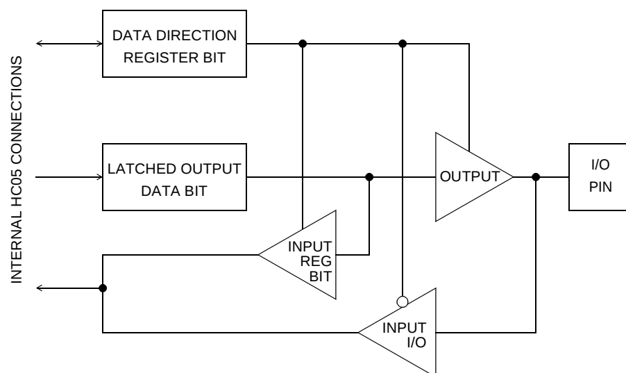
Figure 1-4. I/O Circuitry
