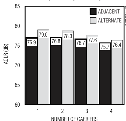
W-CDMA BASEBAND ACLR
