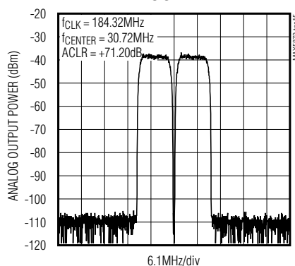
ACLR FOR W-CDMA MODULATION TWO CARRIER
