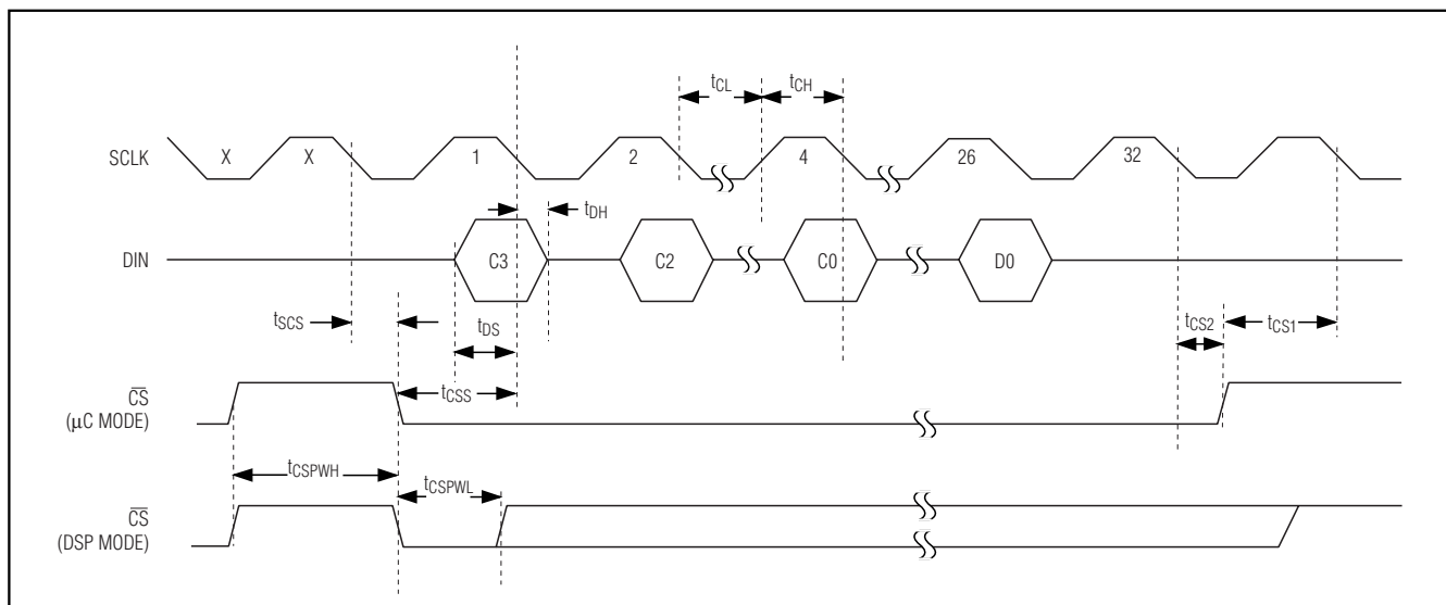
Figure 1. Serial-Interface Timing
