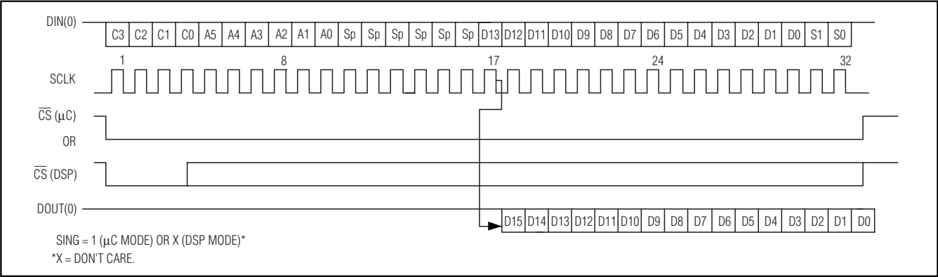
Figure 10. Read Data Timing When Not Daisy Chained
