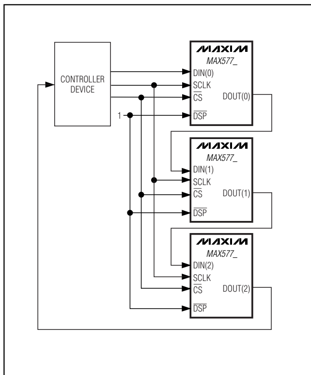
Figure 5. Daisy-Chain Configuration
