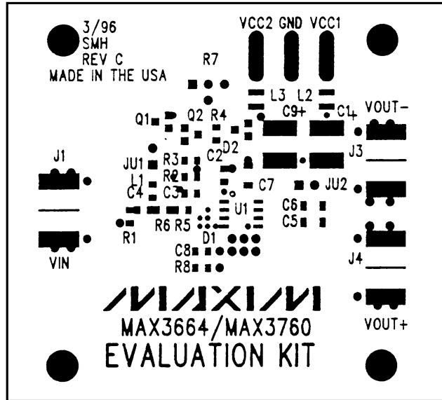
Figure 3. MAX3664 EV Kit Component Placement Guide—Component Side
