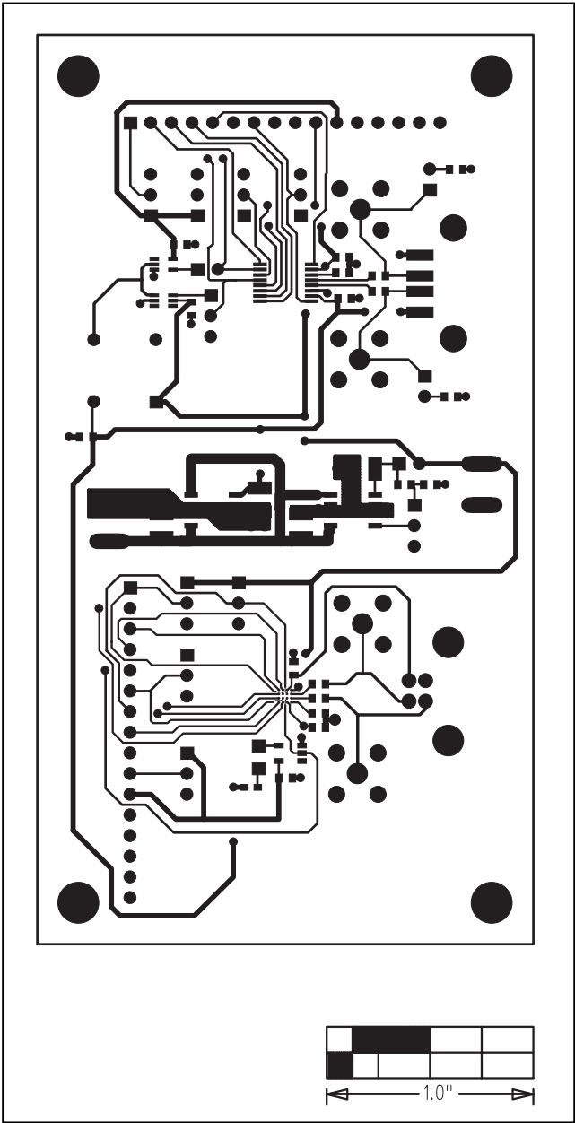
Figure 3. MAX3345E EV Kit PC Board Layout—Component Side
