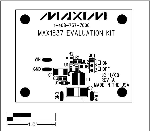
Figure 2. MAX1837 EV Kit Component Placement Guide— Component Side
