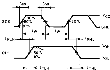
WAVEFORM 1
