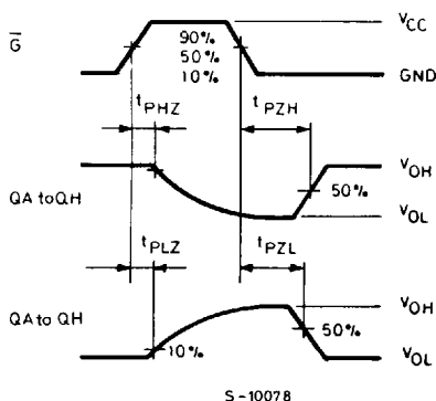
WAVEFORM 6
