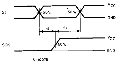
WAVEFORM 5
