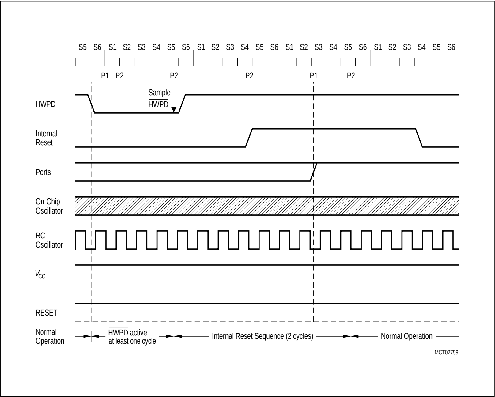
Figure 9-4 Timing Diagram of Hardware Power Down Mode, HWPDP -Pin is active for only one cycle
