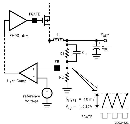
FIGURE 1. Hysteretic Window
