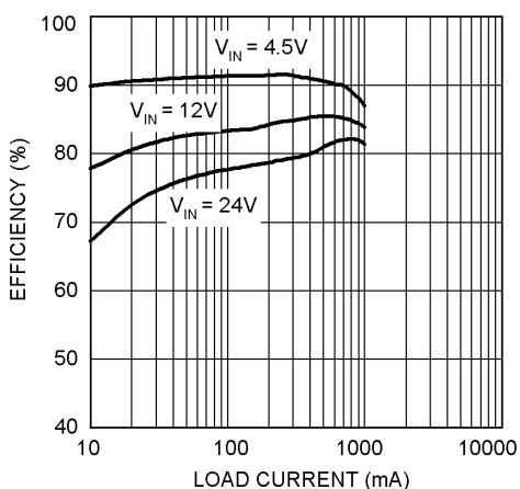
Efficiency vs Load Current (3.3 V_{OUT} , 22 \mu\text{H} )
