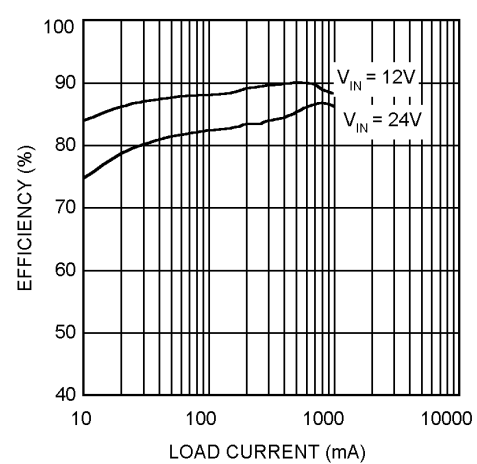
Efficiency vs Load Current (5.0 V_{OUT} , 22 \mu\text{H} )
