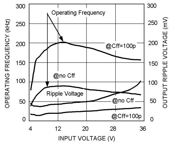
Feed-Forward Capacitor (C ff ) Effect
