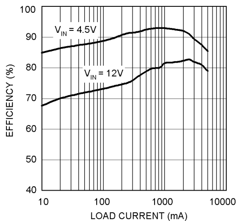
Efficiency vs Load Current (3.3 V_{OUT} , 6.8 \mu\text{H} )
