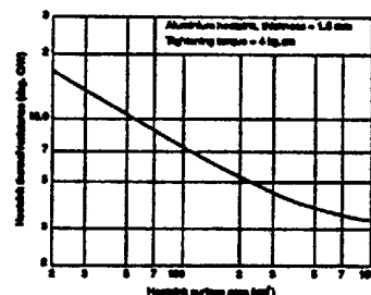
Maximum heatsink thermal resistance vs. surface area
