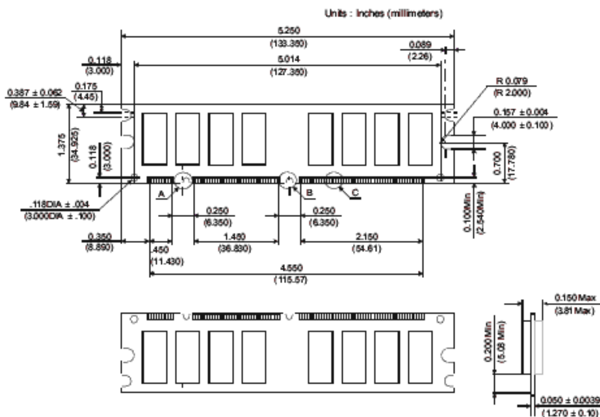
Figure 1: KVR100X64C2/512 168-Pin SDRAM Module
