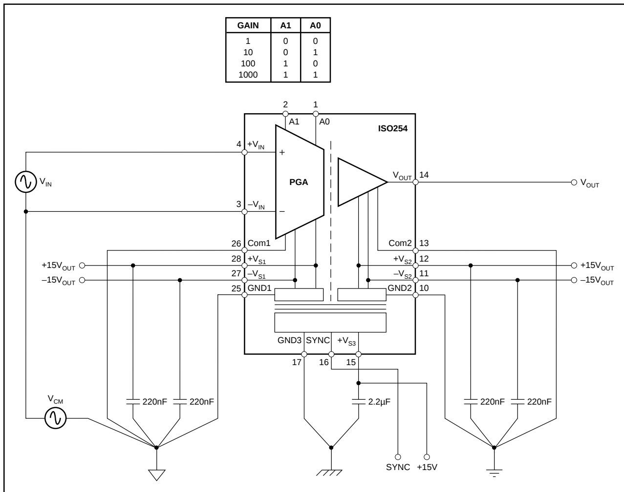
FIGURE 1. Basic Connections.
