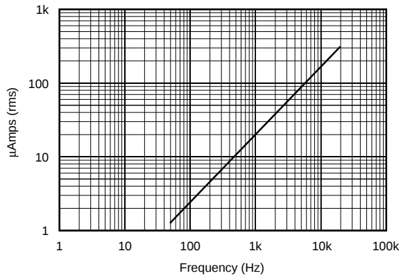
ISOLATION LEAKAGE CURRENT vs FREQUENCY ( V = 240\text{Vrms} )
