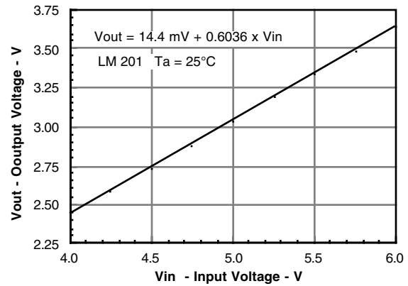
Figure 19. Transfer gain
