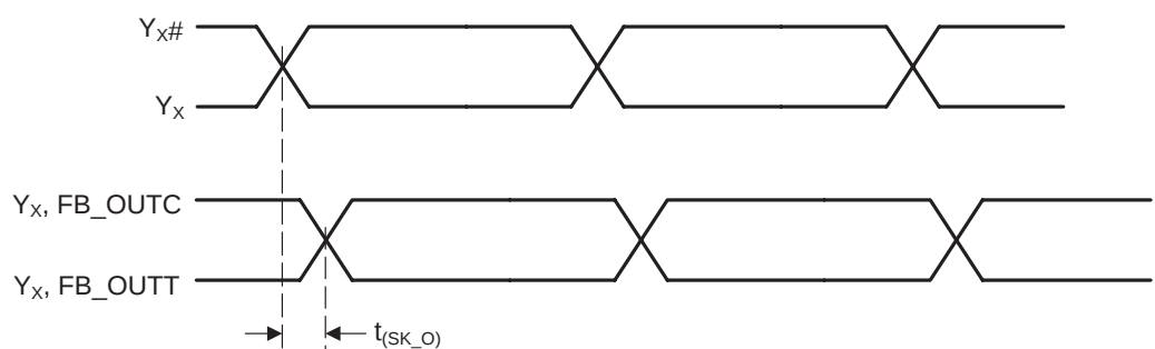
Figure 5. Output Skew
