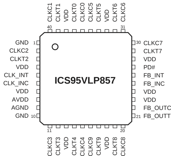
40-Pin MLF
