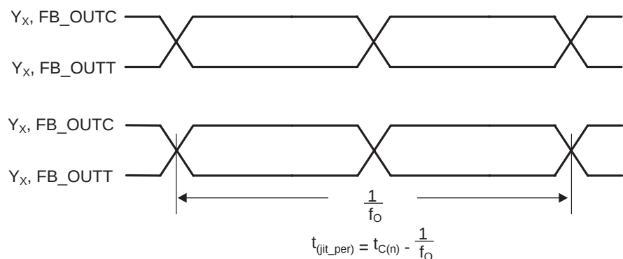
Figure 6. Period Jitter
