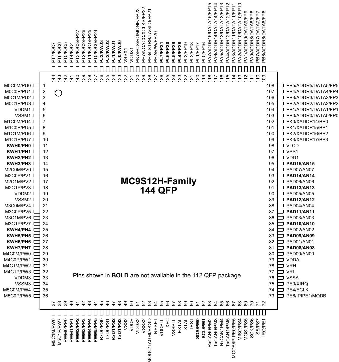
Figure 3. MC9S12H-Family Pin Assignments, 144 Pin QFP package
