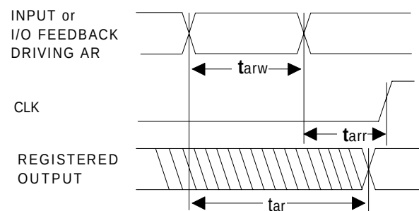
Asynchronous Reset
