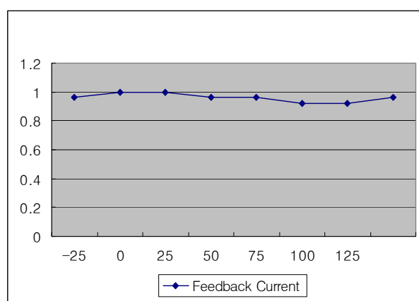
Figure 4. Feedback Source Current vs. Temp
